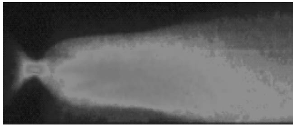
Fig. 6. Temporal scan of the plasma emission for the initial argon pressure of 3.5 mbar and the discharge current of 200 kA; the total scan duration is 6 \mu\text{s} , the transverse size is 2 cm.
